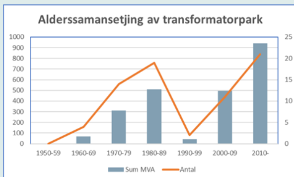
Figur 5 Aldersfordeling, kraftransformatorar
